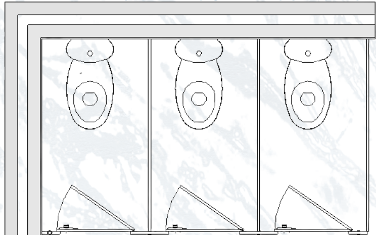
MULTIPLE CORNER CUBICLES
